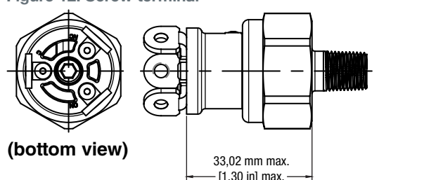
Figure 12. Screw terminal
