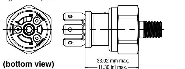
Figure 11. Spade terminal
