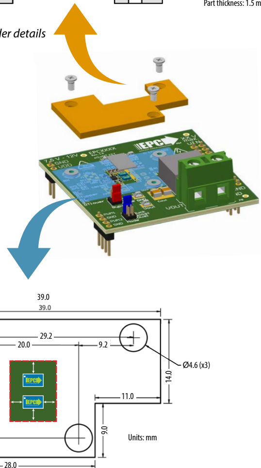
Figure 11: Insulator sheet details with opening for the TIM with location of the FETs
