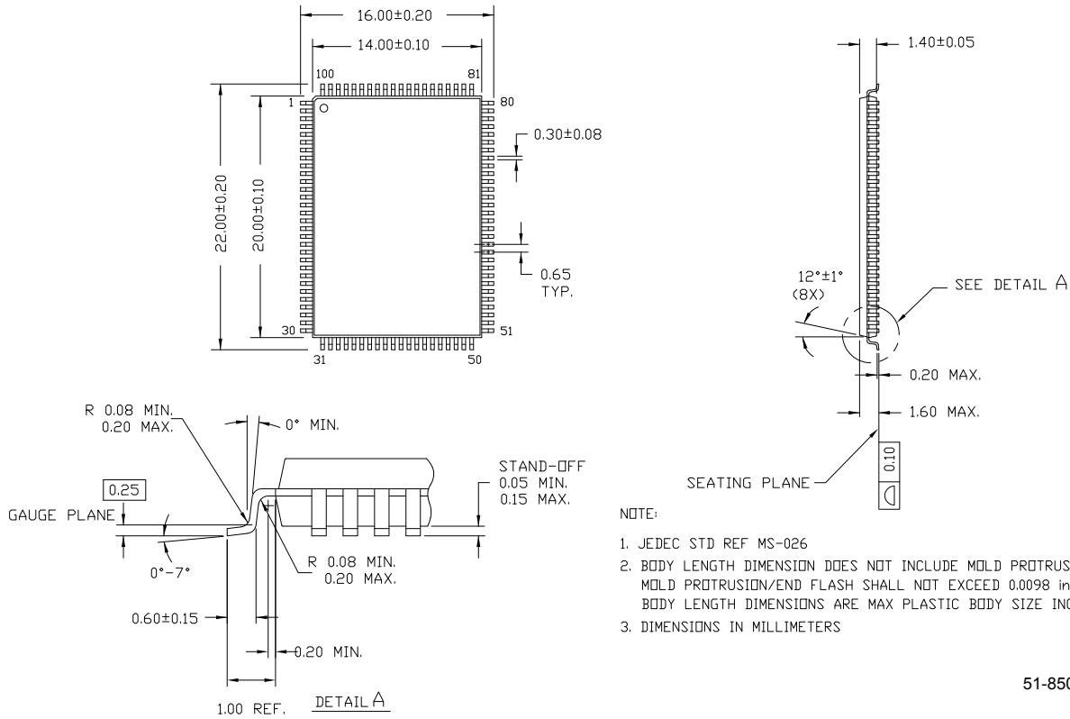
Figure 11. 100-pin Thin Plastic Quad Flatpack (14 × 20 × 1.4 mm) A101
