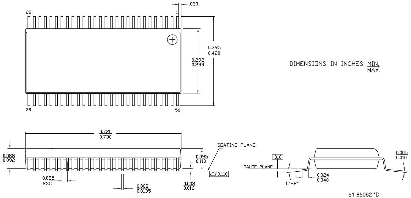
Figure 12. 56-pin Shrunk Small Outline Package 056
