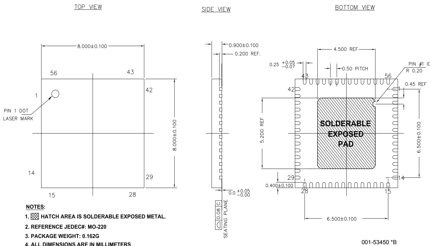
Figure 14. 56-pin QFN (8 × 8 × 0.9 mm) - Sawn
