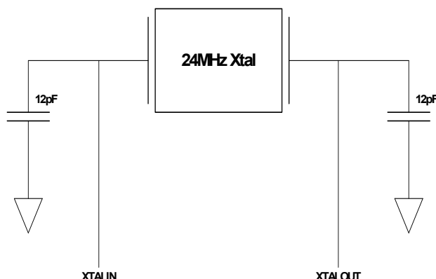
Figure 6. XTALIN/XTALOUT Diagram
