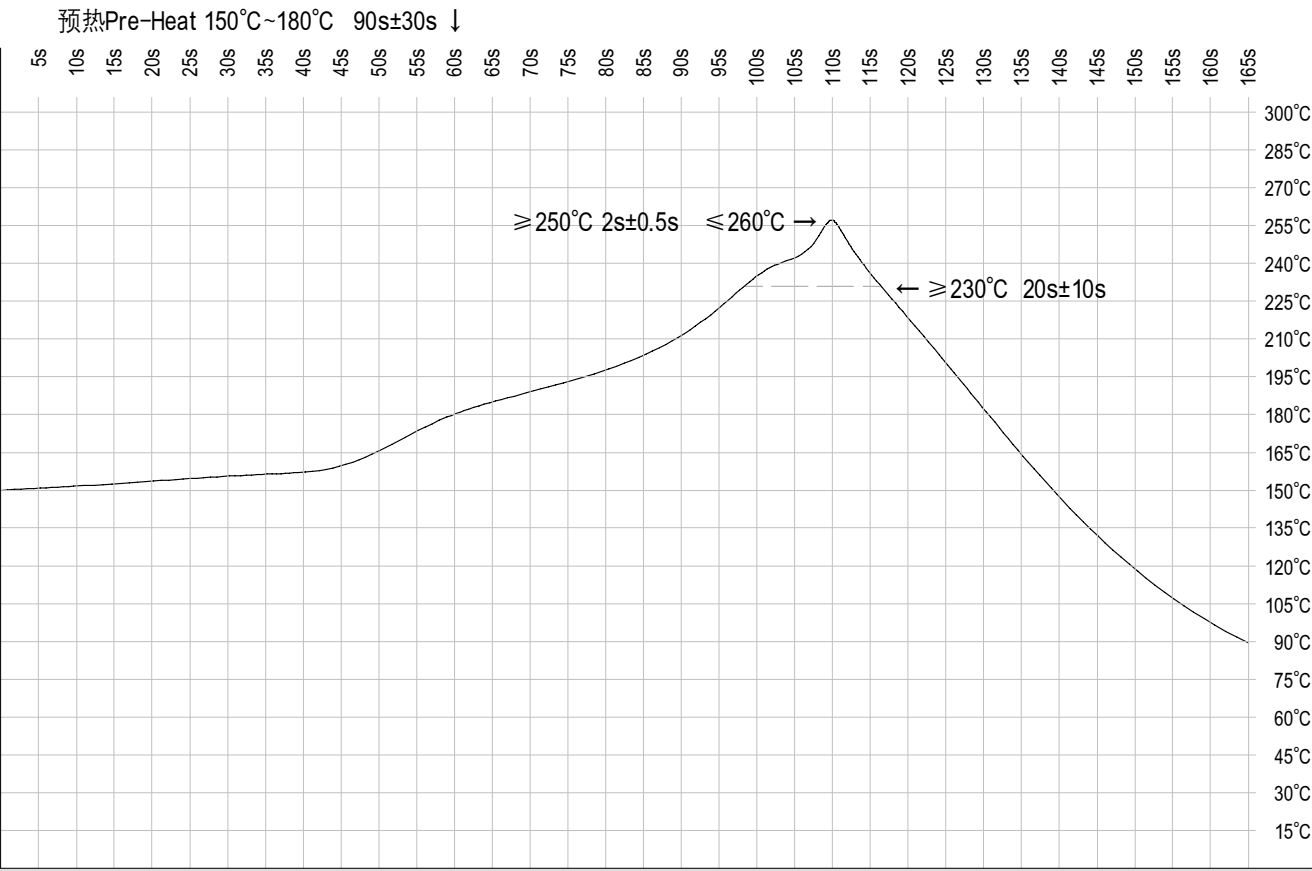
温度条件图 TEMPERATURE CONDITION GRAPH
