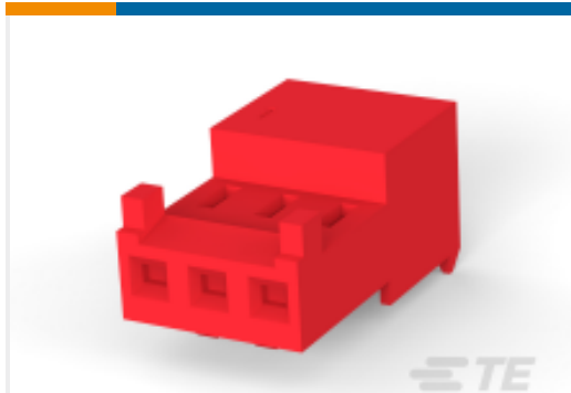
TE Part #3-644563-6 Nylon Tin Plated Receptacle: 2.54 mm, with Mating Alignment, MTA 100
