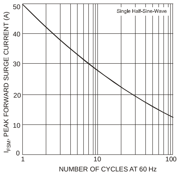
Fig. 6 Max Non-Repetitive Peak Forward Surge
