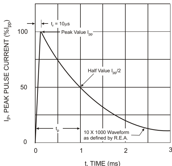
Fig. 2 Pulse Waveform
