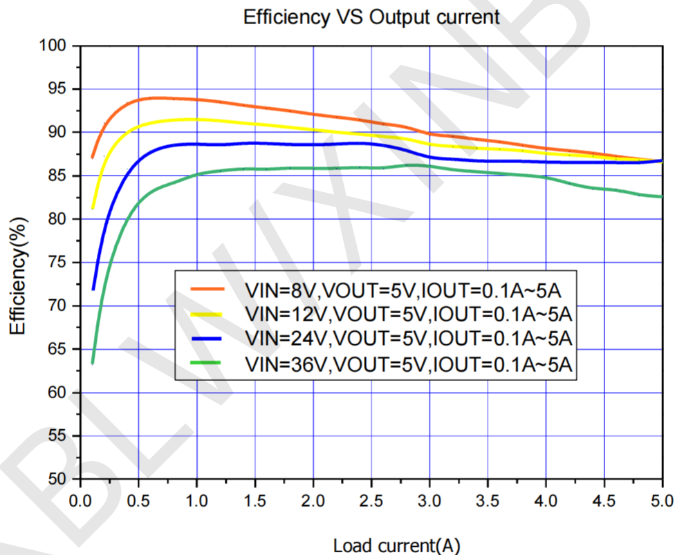
Figure 3. XBL4015 System Efficiency Curve
