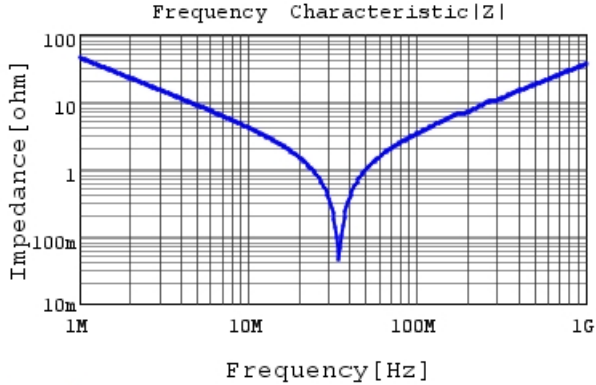
RCE5C2J392J2K1H03B |Z| DCOV, 25degC
