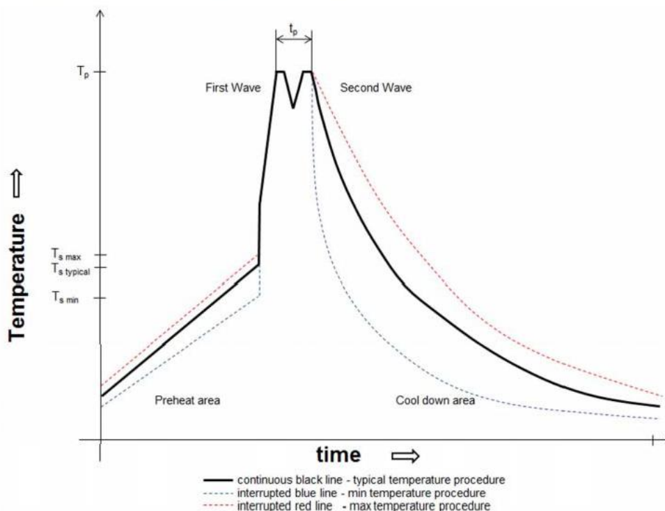
Classification Wave Soldering Profile:
