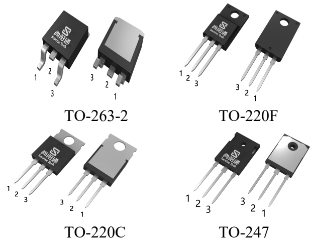
Figure 2 Package Types of SRC65R145B
