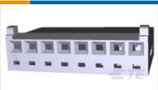
TE Part #1375820-8 CST-100 II HOUSING 8 POS
