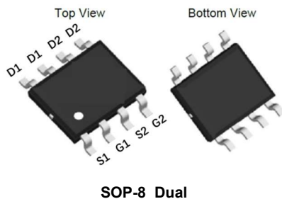
SOP-8 Dual
