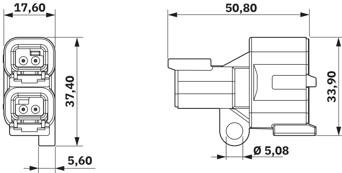
ATM04-2P-P007 top view and side view
