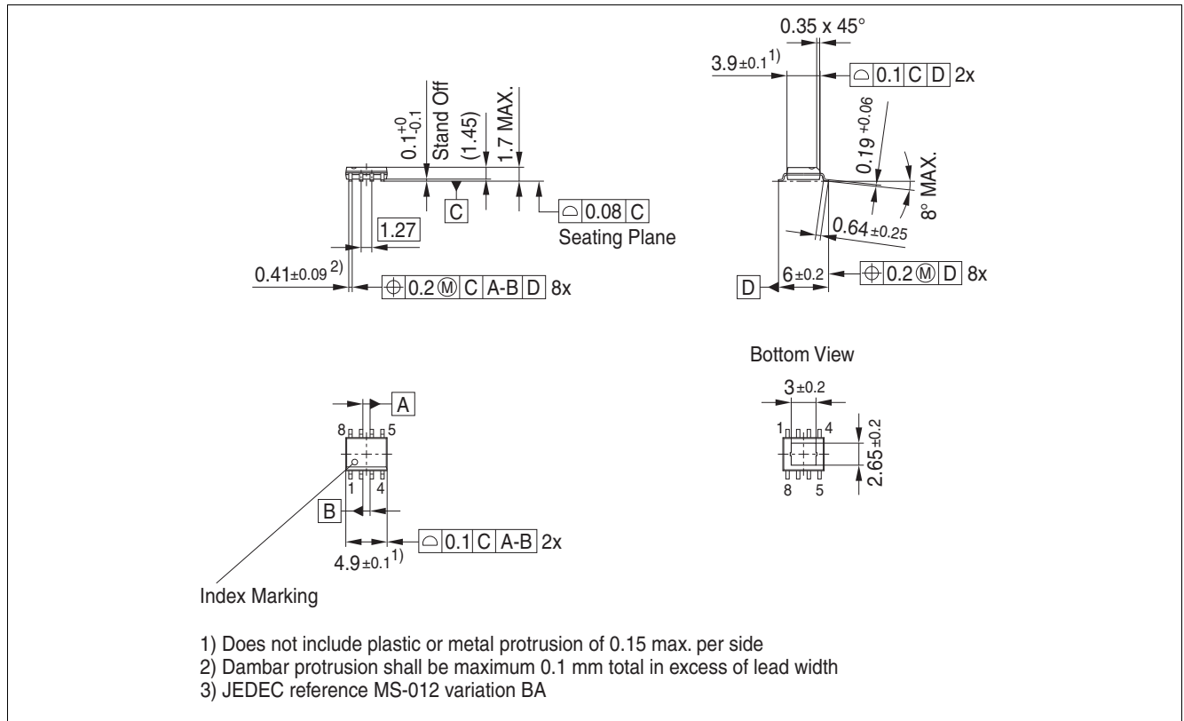
Figure 8 PG-DSO-8 EP
