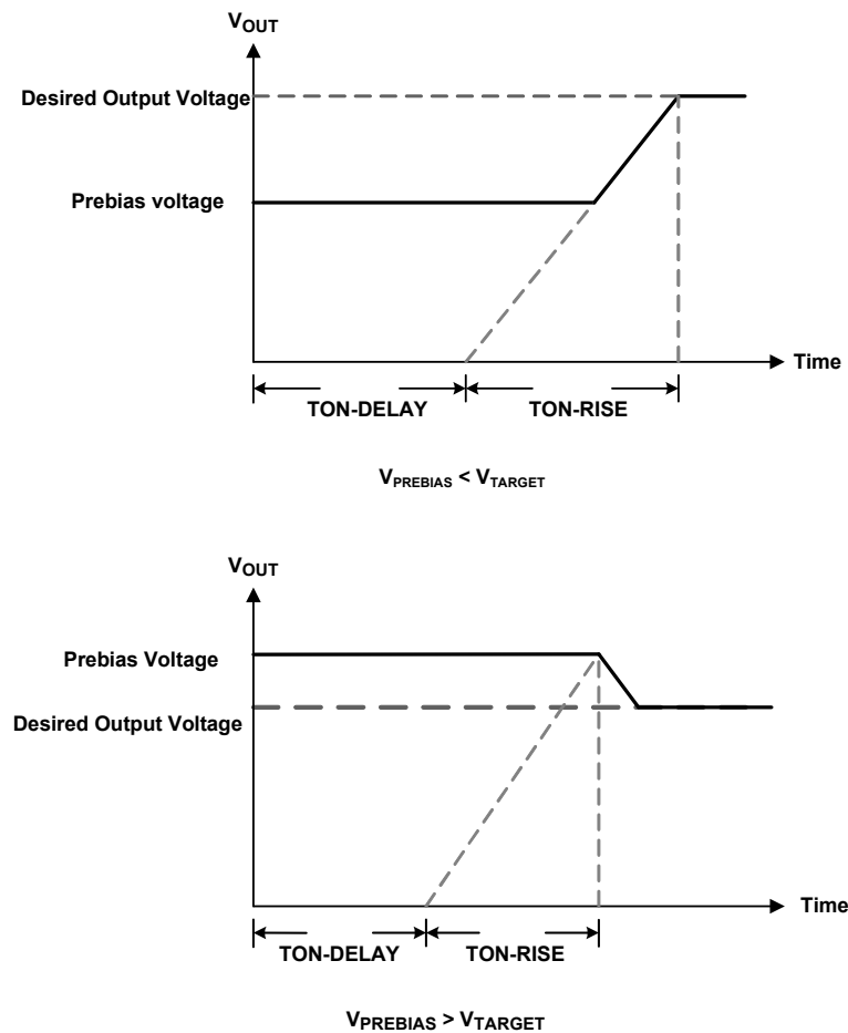
Figure 31. Output Responses to Prebias Voltages
