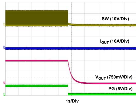
Figure 14. Single Channel Shutdown 12V IN , 1.5V OUT , 0A
