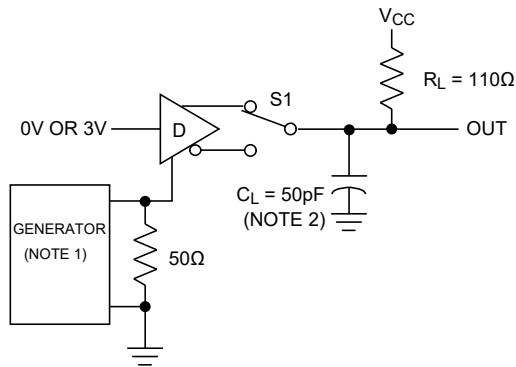
Figure 6. Enable and Shutdown Times ( t_{PZL} , t_{PSL} , t_{PLZ} )
