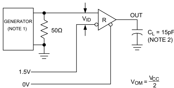
Fig. 7 Receiving Transmission Delay
