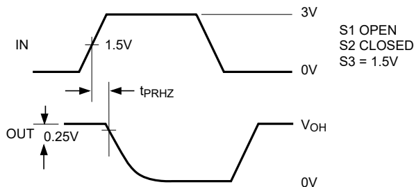
Figure 8 Receiving OPEN and CLOSE Times
