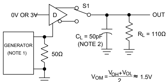
Figure 5. Enable and Shutdown Times ( t_{PZH} , t_{PSH} , t_{PHZ} )
