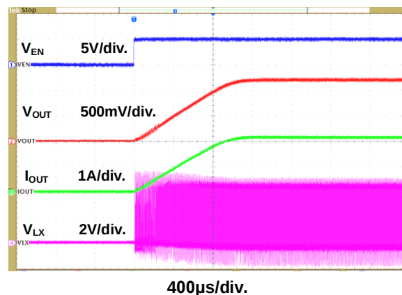
Figure 13. Power On through EN Waveform
