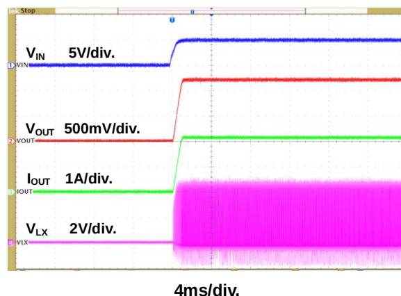
Figure 9. Power On through VIN Waveform
