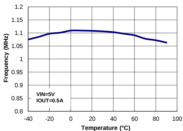
Figure 7. Frequency vs. Temperature
