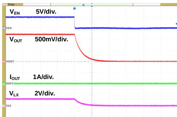
Figure 14. Power Off through EN Waveform
