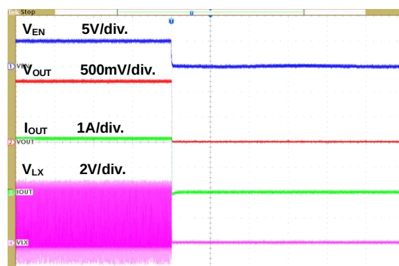
Figure 15. Power Off through EN Waveform
