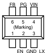
Figure 1. Pin Assignment of TD8002X
