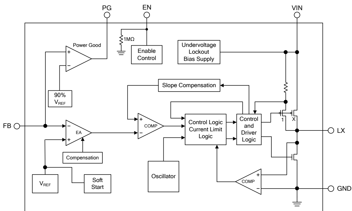
Figure 3. Block Diagram of TD8002X
