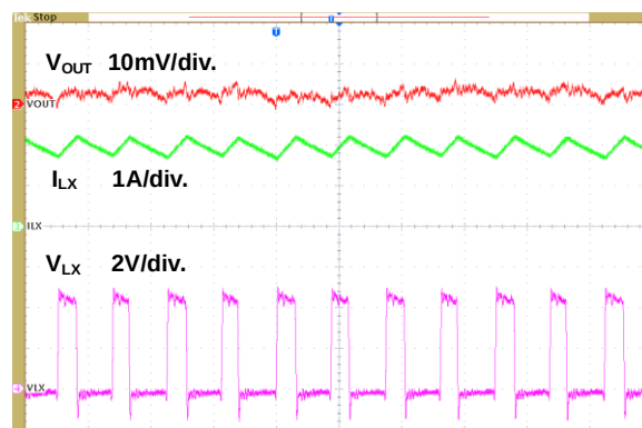
Figure 17. Steady State Waveform
