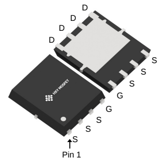
DFN5X6-8L (DFN-8-EP(6.1x5.2))
