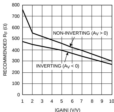
Figure 24. Recommended R_F vs. Gain
