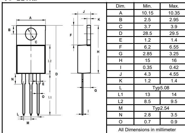
T0-220AB
