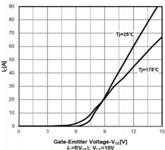
Typ. Transfer characteristics
