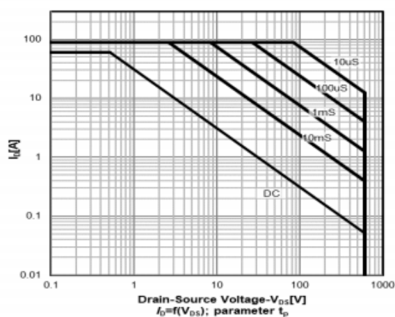
Safe operating area Ta=25 °C Full PAK
