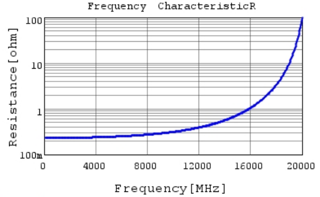
GJM1555C1H1R0CB01 R DCOV,25degC
