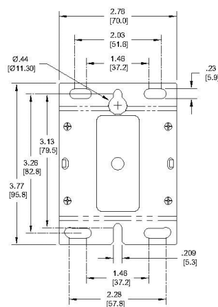
4 Pole Contactor
