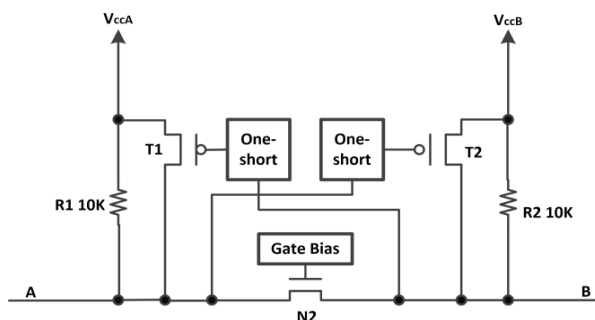
Architecture of TXS0104E
