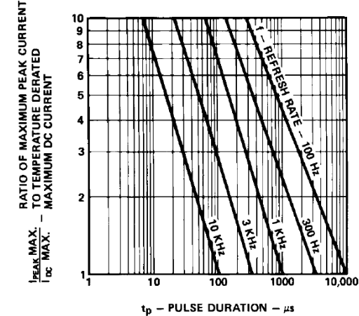
Figure 5: Maximum Tolerable Peak Current vs. Peak Duration. I PEAK MAX. determined from temperature derated I DC MAX.
