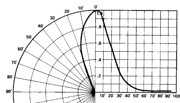
Figure 9: Relative Luminous Intensity vs. Angular Displacement, HLMP-K105
