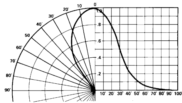
Figure 7: Relative Luminous Intensity vs. Angular Displacement, HLMP-K101
