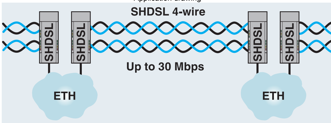
Linear structure (4-wire)
