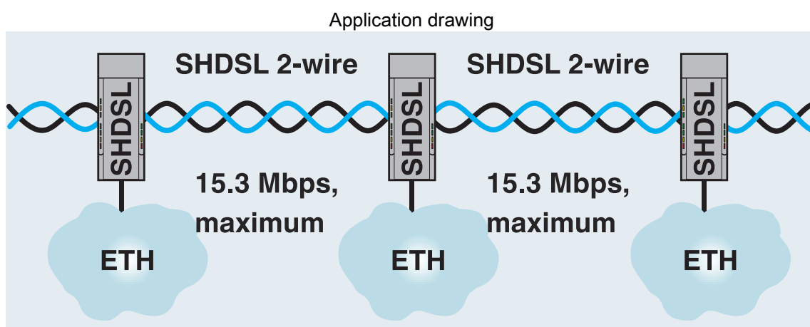
Linear structure (2-wire)
