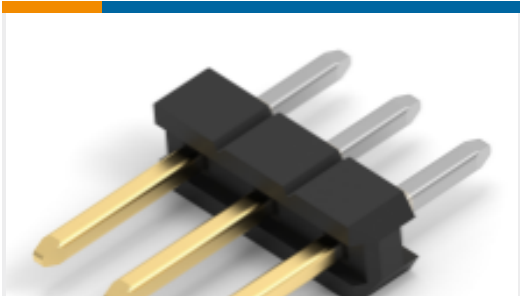
TE Part #2355177-3 3P,2MM,BRK HDR,SRVT,2.8,0.38AU,TB
