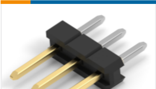
TE Part #2355177-4 4P,2MM,BRK HDR,SRVT,2.8,0.38AU,TB
