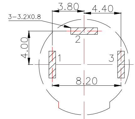
PCB.WELDING DRAWING
