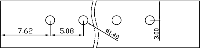
PCB Layout
