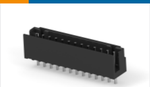
TE Part #292161-8 CT 2mm Post Header Asmbly: Box V DIP
