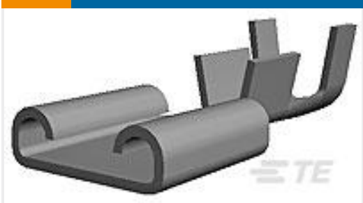
TE Part #6-160432-3 250 FASTON REC 20-16 AWG NPST
