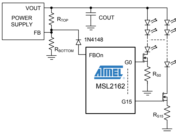
Figure 4. FBO connects to the Power Supply Voltage Divider Through a Diode
