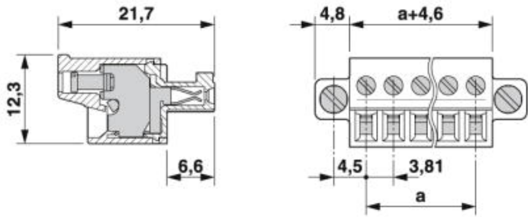
Dimensional drawing
