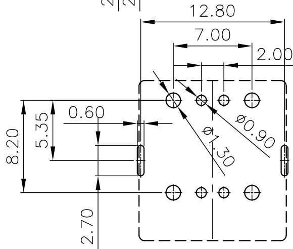
P. C. B LAYOUT
