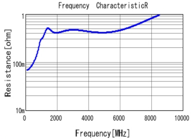
■ GRM0335C1E561GA01 R DC0V, 25degC
