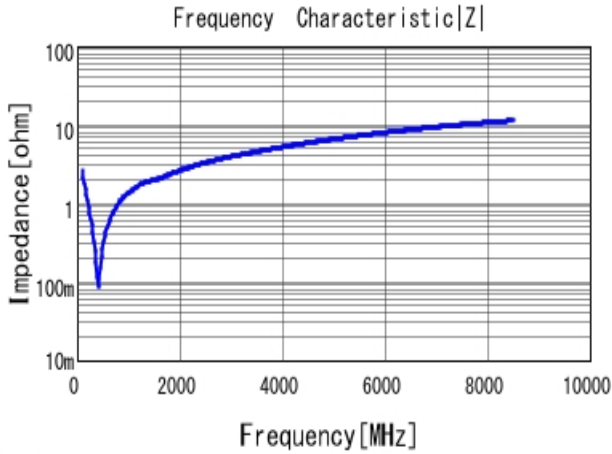
■ GRM0335C1E561GA01 |Z| DC0V, 25degC
