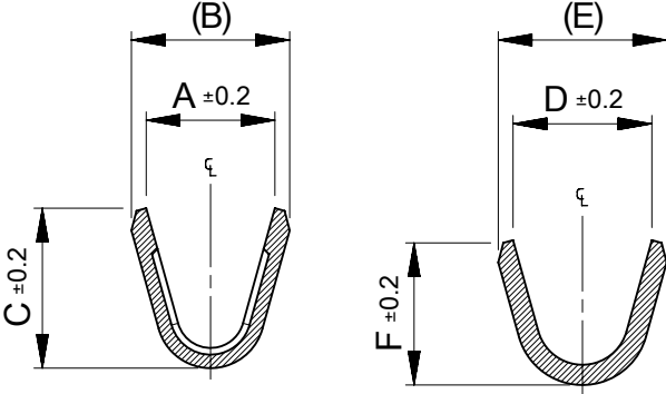
SECTION Z-Z SECTION Y-Y
