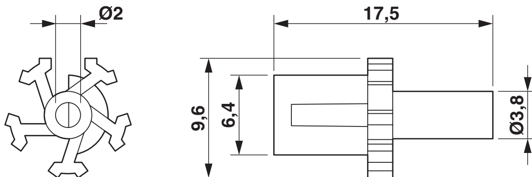
Dimensional drawing
