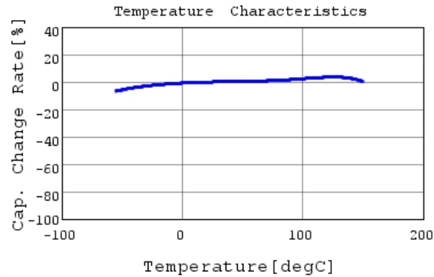
GCJ188R92A682KA01 C-Temp. capchange, DC0.0V,
