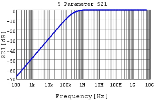
GCJ188R92A682KA01 S21 DC0V,25degC
