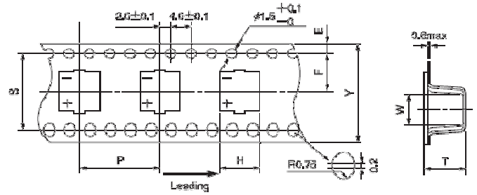
Fig. 1-2 Carrier tape \phi D \geq 12.5
