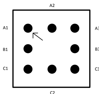
Figure 1. 8-bump DSBGA
