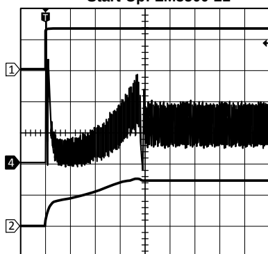
Start-Up: LM3500-21
