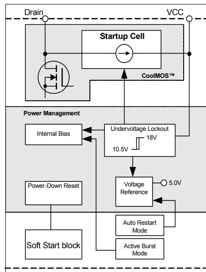
Figure 3 Power Management
