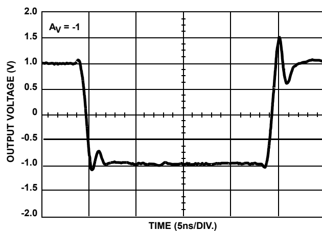
FIGURE 8. LARGE SIGNAL PULSE RESPONSE
