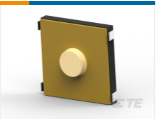
TE Part #2337235-1 TACT MICRO JB 4.6X4.4X1.05 P3.5 PH 100GF
