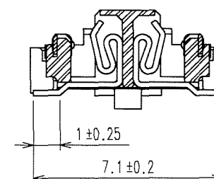
CROSS CUT SECTION - SIGNAL ( 5 : 1 )
