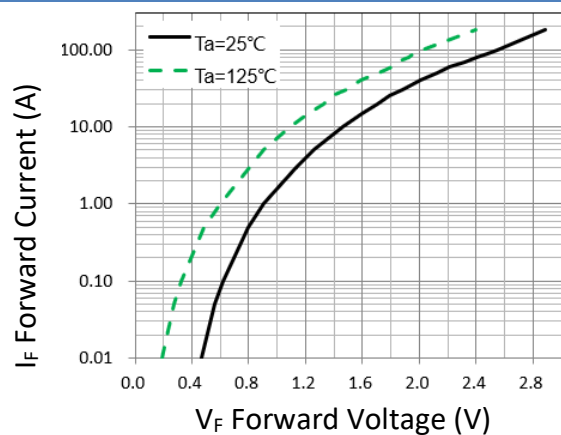
Figure 1. Forward Characteristic(typ.)
