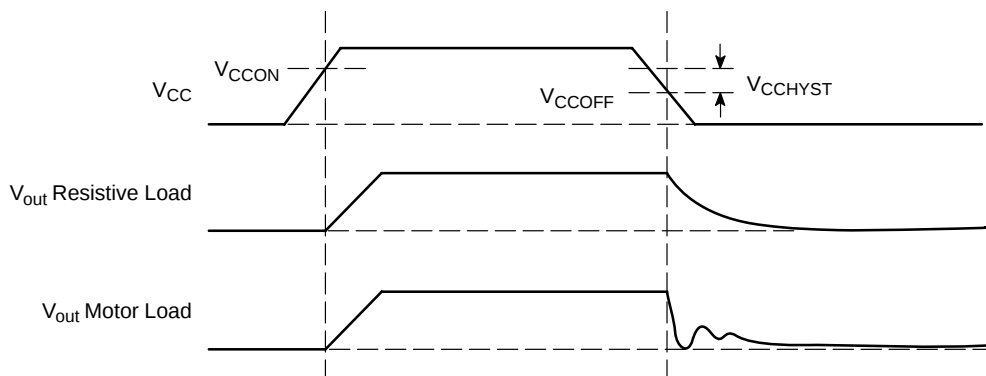
Figure 14. Timing Diagram
