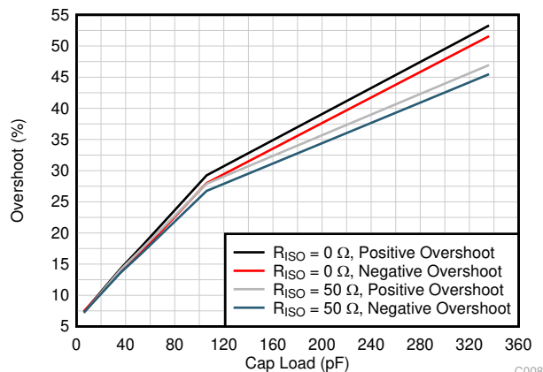
Figure 7-6. Small-Signal Overshoot vs Capacitive Load (100-mV Output Step, G = 1)
