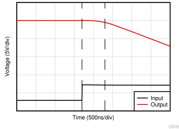
Figure 6-30. Positive Overload Recovery
