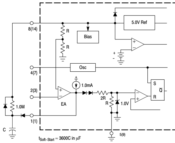
Figure 24. Soft-Start Circuit
