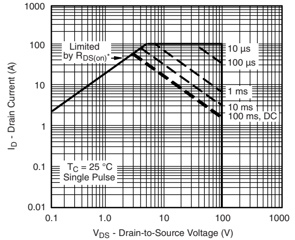
* V_{GS} > \text{minimum } V_{GS} \text{ at which } R_{DS(on)} \text{ is specified} Safe Operating Area, Junction-to-Case
