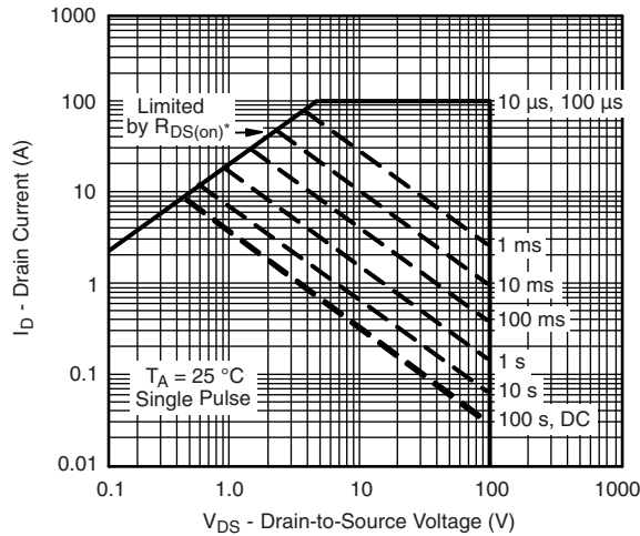
* V_{GS} > \text{minimum } V_{GS} \text{ at which } R_{DS(on)} \text{ is specified} Safe Operating Area, Junction-to-Ambient
