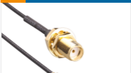
TE Part #CSH-SGFB-200-UFFR SMA to U.FL/MHF1 200mm 1.32 OD
